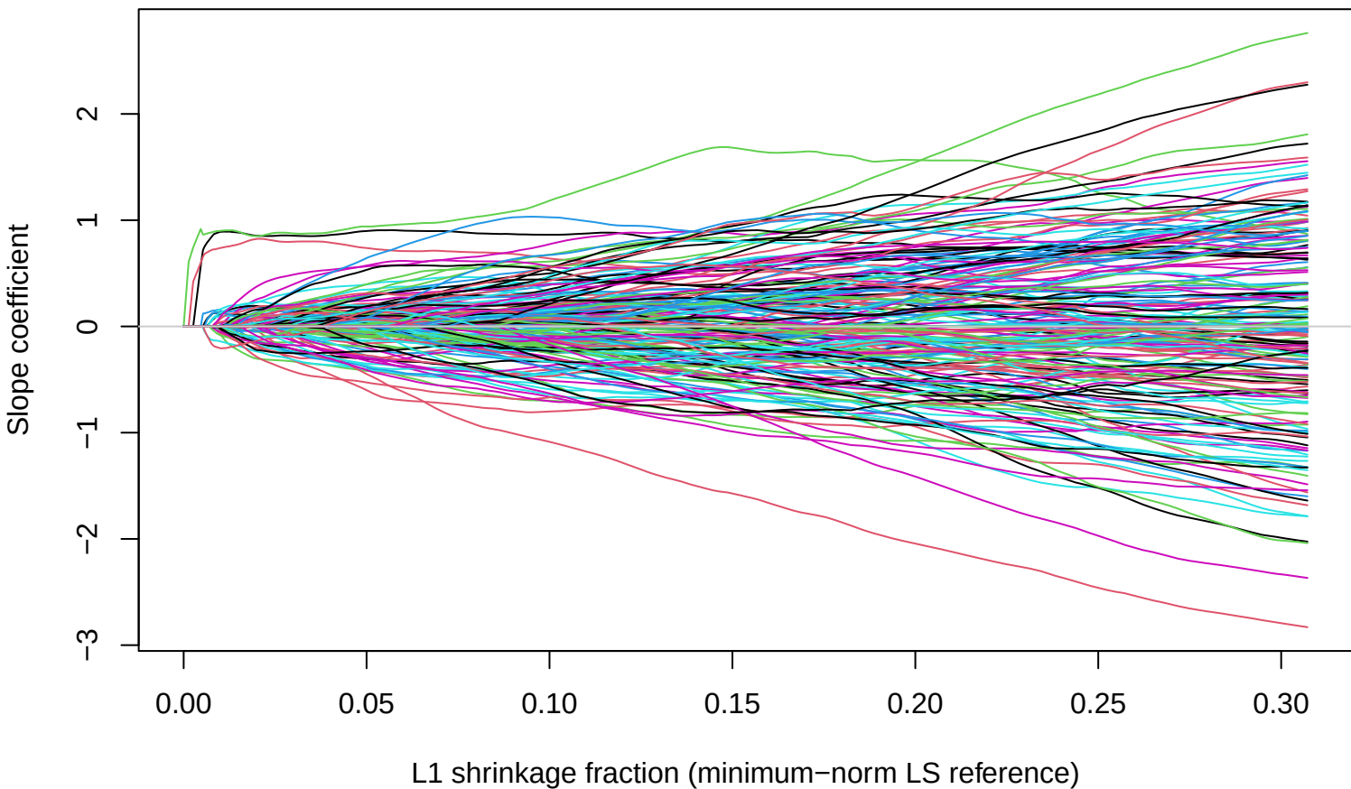
lasso coefficient path: p = 200
